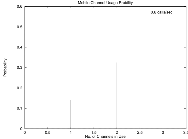
Figure 4: Channel Usage Prob. Density Function for 0.6 Call/Sec.
